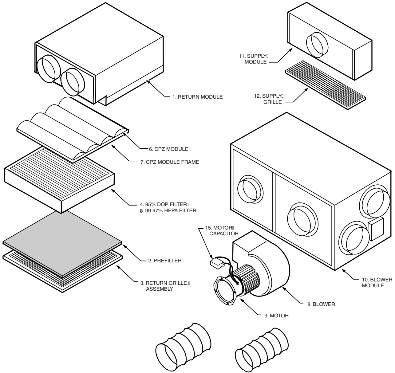
Fig. 11. F120 exploded view.
